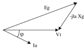
Figure 2. Vector diagram of over excitation conditions
