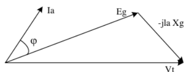
Figure 1. Vector diagram of under excitation conditions
