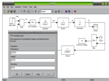
Figure 9. MATLAB simulation model with PID controller
