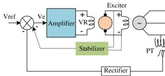
Figure 3. AVR Model
